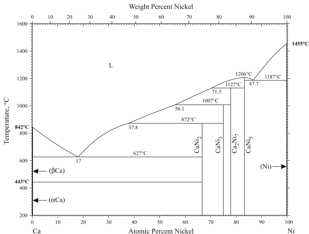
Fig. 1 Ca-Ni phase diagram
